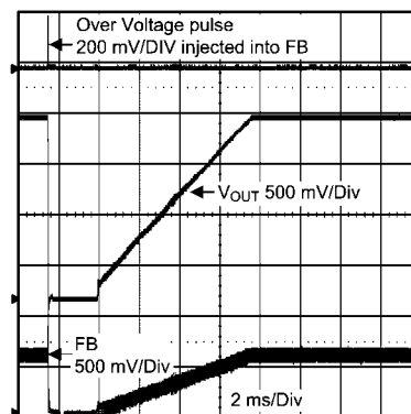
Over-Voltage Fault
