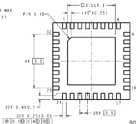
32-Lead LLP Package NS Package Number SQA32A
