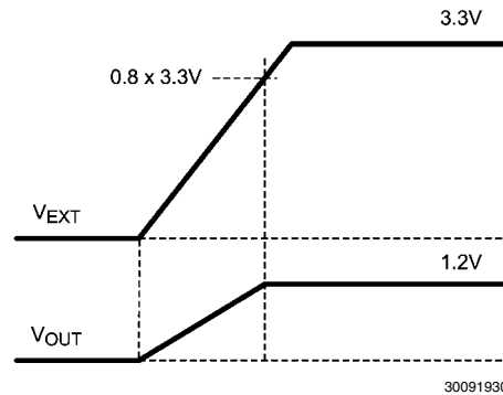
FIGURE 9. Tracking an External Supply
