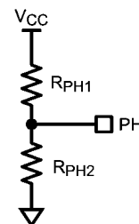
FIGURE 5. Phase Selection
