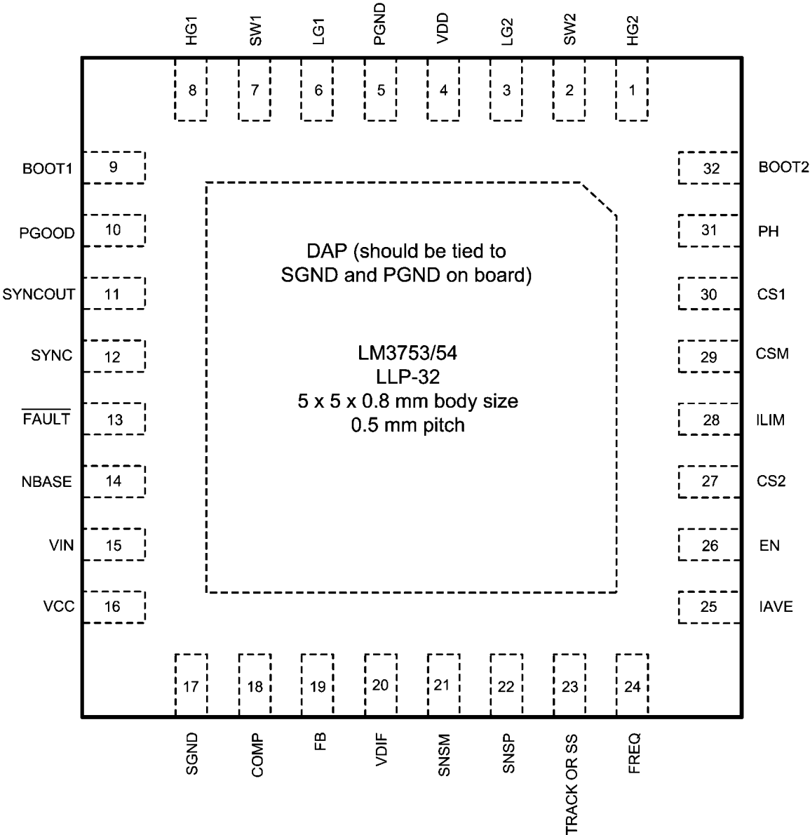
Top View 32-Lead LLP
