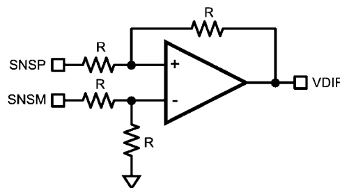
FIGURE 7. Differential Amplifier
