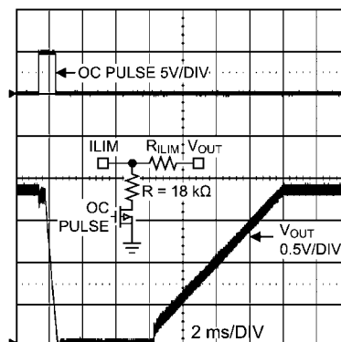
Over-Current Fault (Soft Short)
