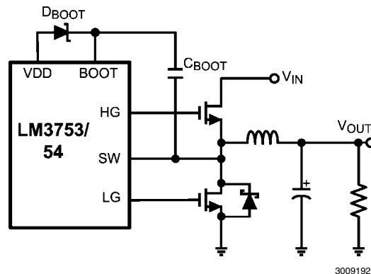
FIGURE 6. Bootstrap Circuit
