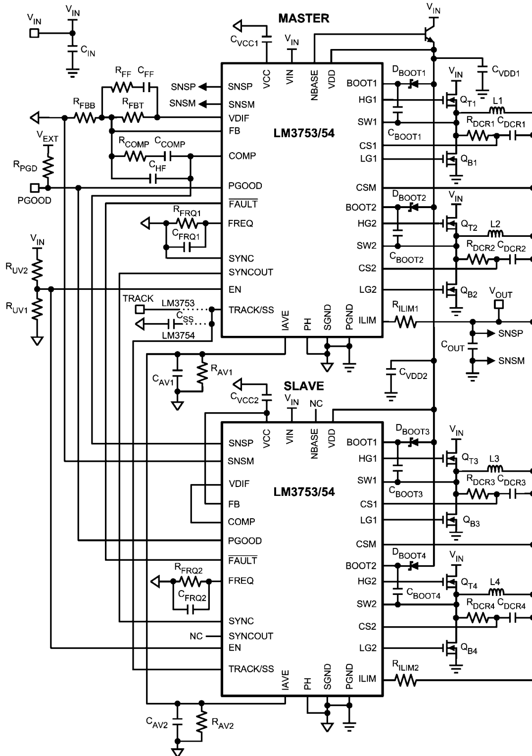
FIGURE 20. Typical Application
