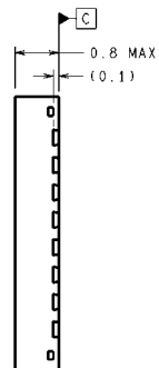
32-Lead LLP Package NS Package Number SQA32A
