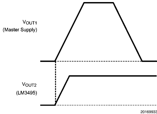
FIGURE 3. Tracking with Equal Slew Rates
