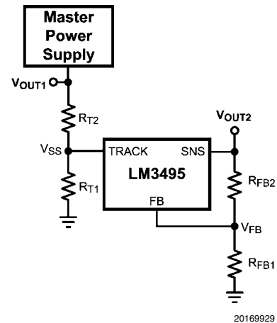
FIGURE 1. Tracking Circuit
