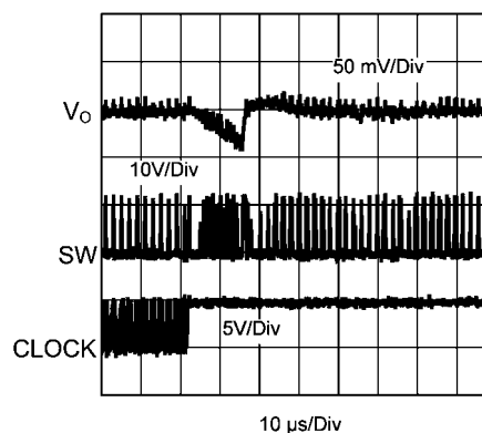
SYNC to FA Transition Clock Ends on Logic High BOM in Table 1
