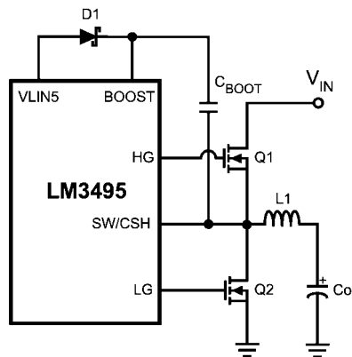
FIGURE 5. Bootstrap Circuit
