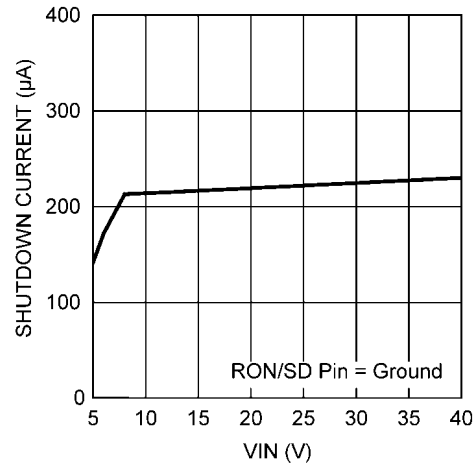
Shutdown Current into V_{IN}
