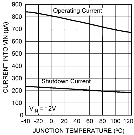
Operating & Shutdown Current vs. Temperature
