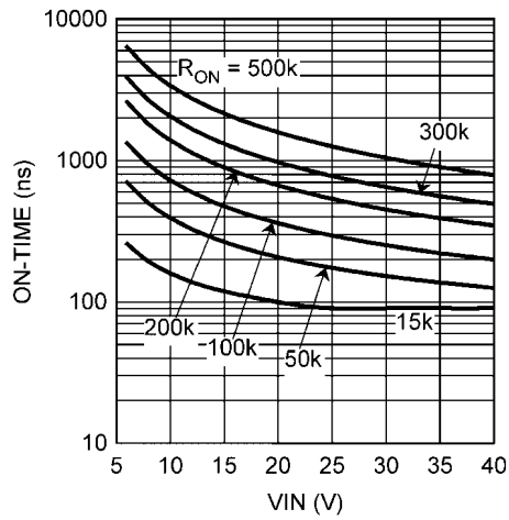
ON-TIME vs. V_{IN} and R_{ON}
