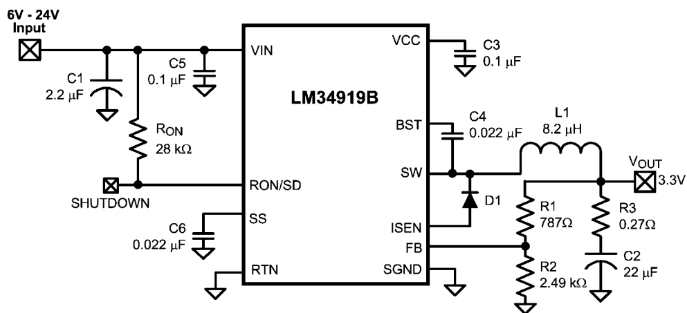
FIGURE 5. Example Circuit
