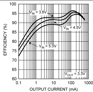
Figure 14. Efficiency vs. Output Current
