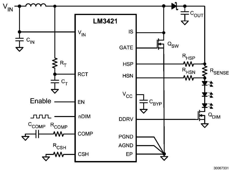
FIGURE 10. LM3421 Boost Topology with High Speed Dimming
