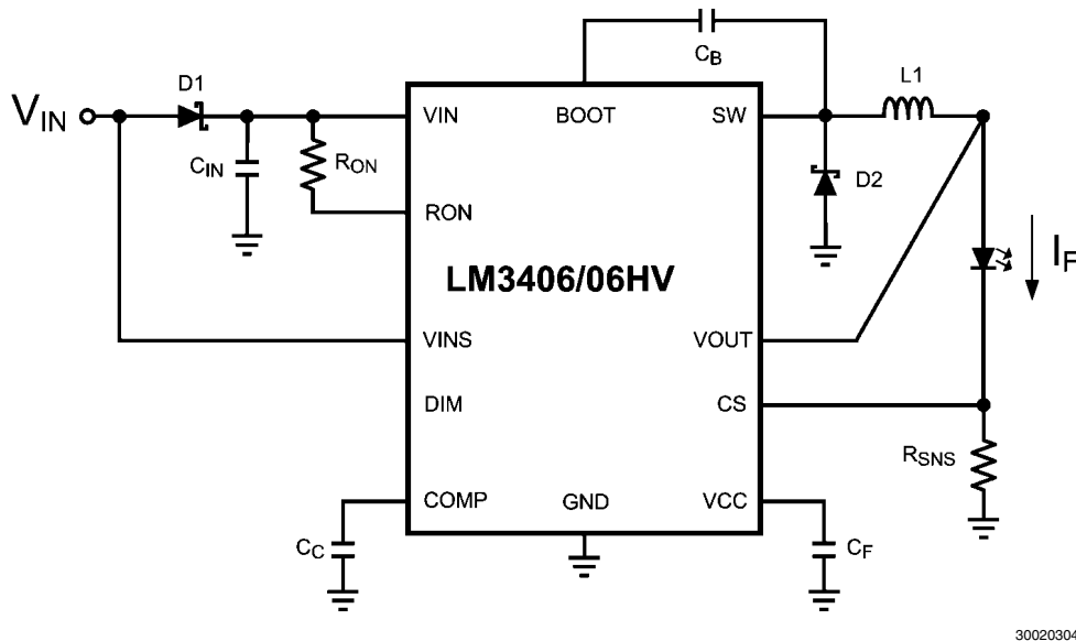
FIGURE 2. Typical Application using Two-Wire Dimming
