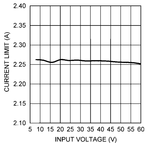
Current Limit vs V_{IN} , LM3406HV
