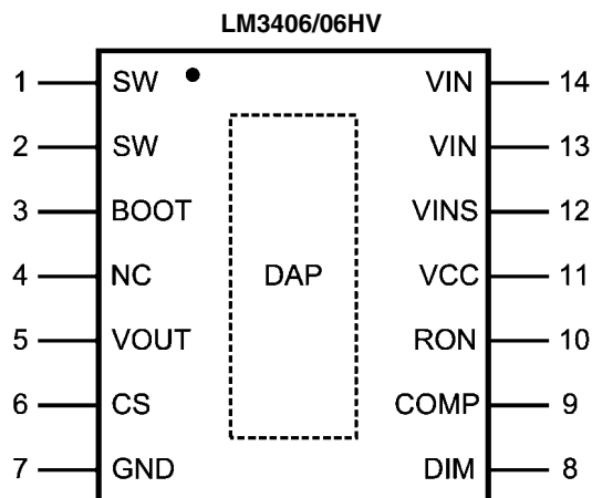
14-Lead Exposed Pad Plastic TSSOP Package NS Package Number MXA14A
