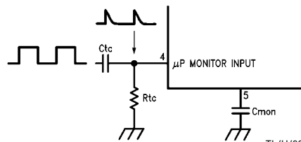
FIGURE 2. Monitoring Square Wave \mu P Signals
