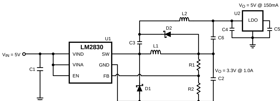
Figure 28. LM2830X (1.6 MHz): Vin = 5 V, Vo = 3.3 V at 1.0 A and LP2986-5.0 at 150-mA Schematic
