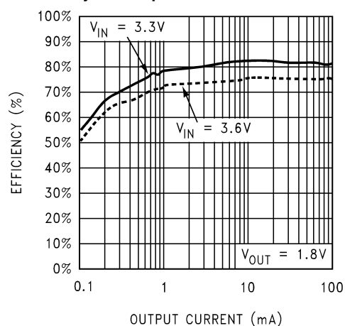
Efficiency vs. Output Current: LM2788-1.8
