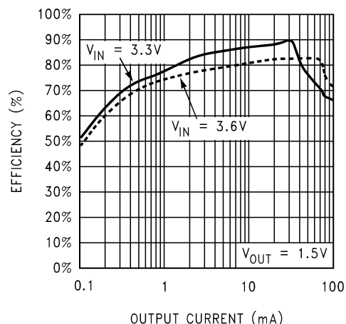
Efficiency vs. Output Current: LM2788-1.5
