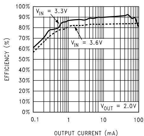
Efficiency vs. Output Current: LM2788-2.0
