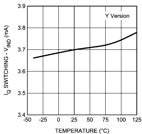
I_Q (Quiescent Current Switching) - "Y"
