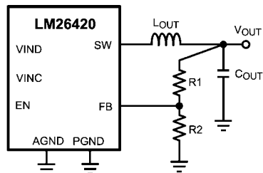
FIGURE 5. Programming V_{OUT}
