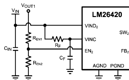
FIGURE 7. V_{OUT1} controlling V_{OUT2} with resistor divider.
