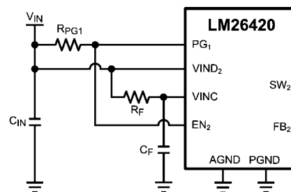
FIGURE 8. PG_1 controlling V_{OUT2} .
