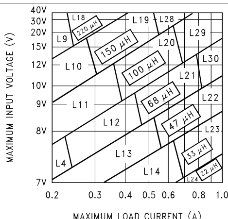
Figure 28. LM2595 5-V
