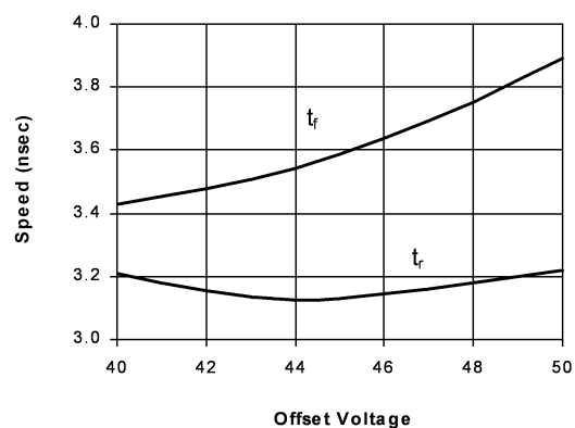
FIGURE 7. Speed vs Offset
