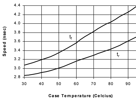
FIGURE 4. Speed vs Temp.
