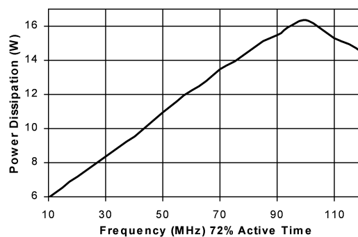
FIGURE 6. Power Dissipation vs Frequency
