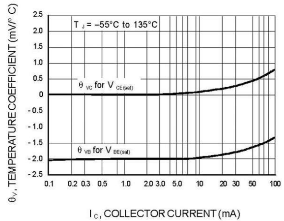
Figure 5. Temperature Coefficients
