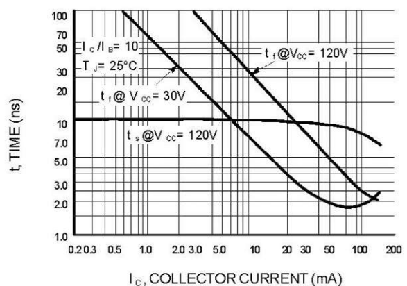
Figure 9. Turn-Off Time
