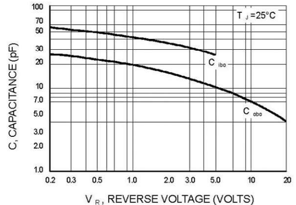
Figure 7. Capacitances
