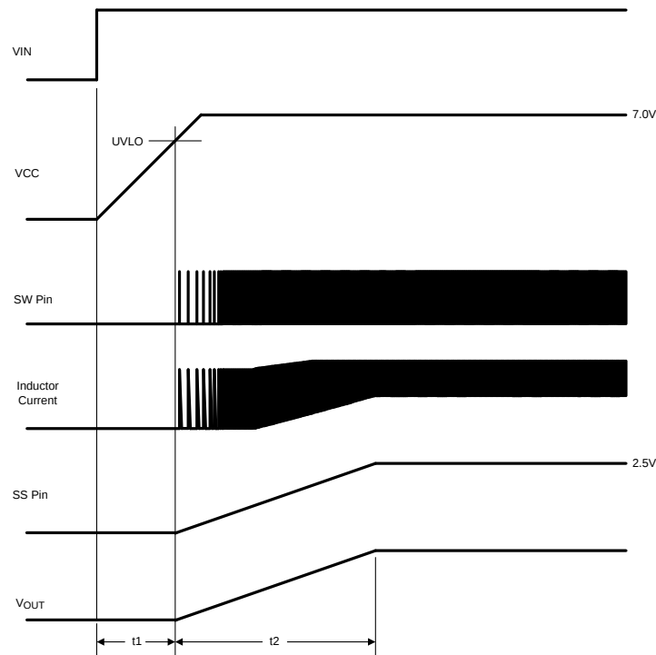
Figure 7. Startup Sequence
