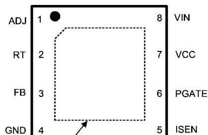
Exposed Pad on Bottom Connect to Ground
