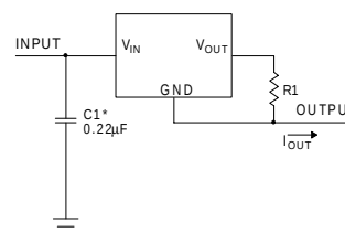
Current Regulator
