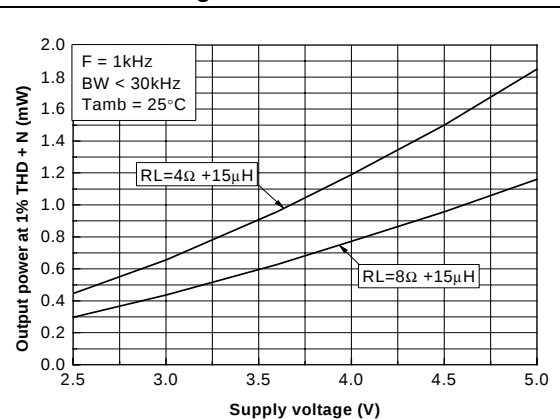
Figure 31. Output power vs. power supply voltage
