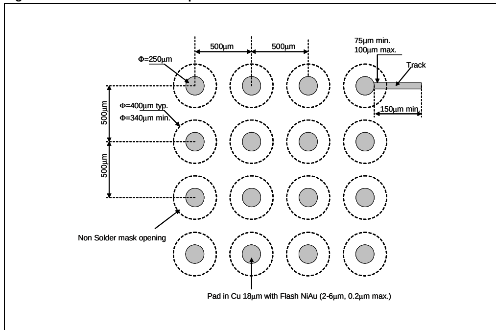
Figure 45. Recommended footprint
