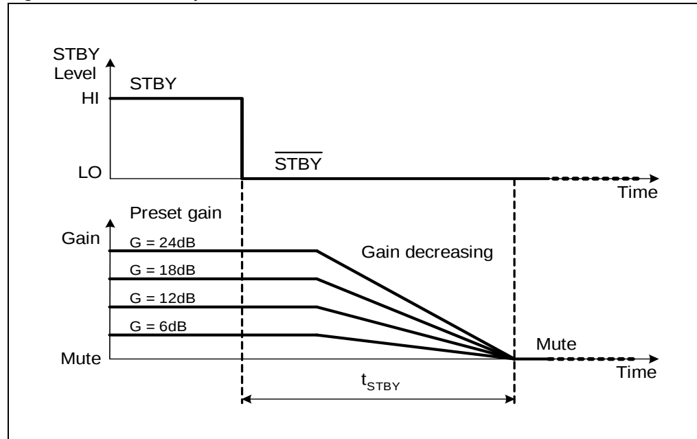
Figure 38. Shutdown phase
