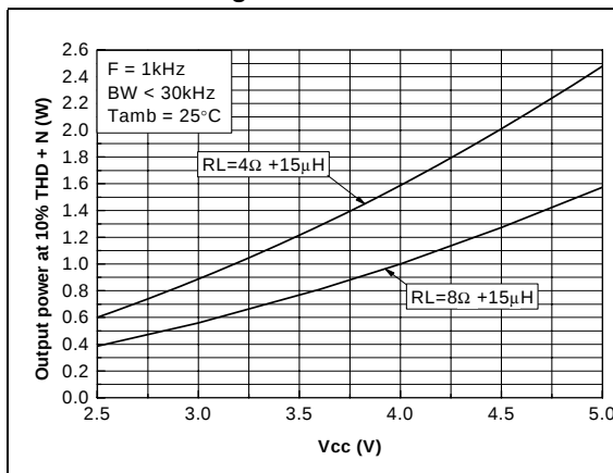
Figure 32. Output power vs. power supply voltage
