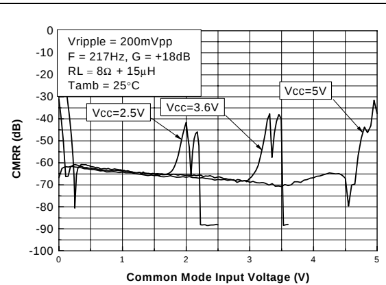
Figure 23. CMRR vs. common mode input voltage
