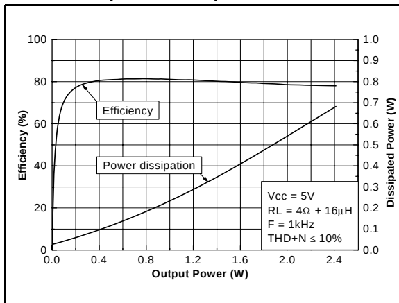
Figure 8. Efficiency vs. output power (one channel)
