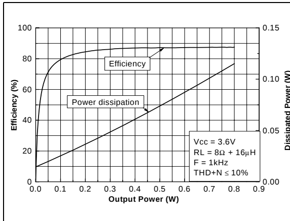
Figure 10. Efficiency vs. output power (one channel)
