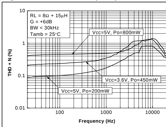
Figure 28. THD+N vs. frequency
