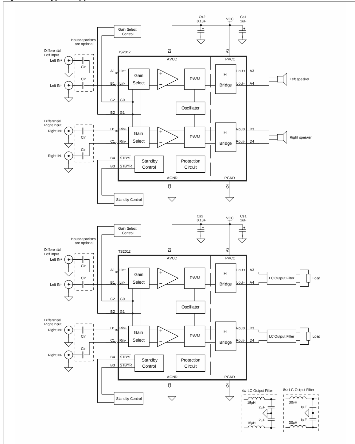
Figure 1. Typical application schematics
