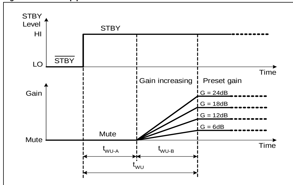
Figure 37. Wake-up phase.
