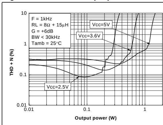
Figure 26. THD+N vs. output power
