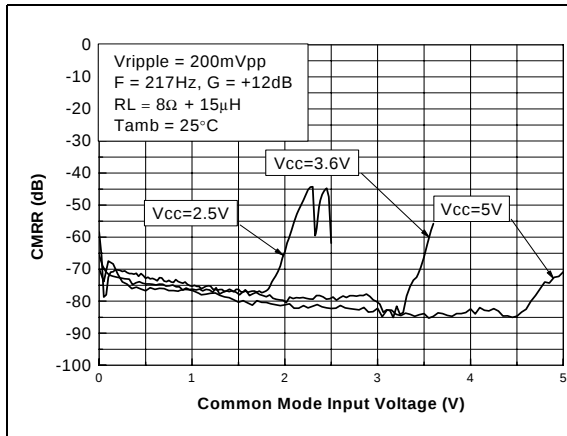
Figure 22. CMRR vs. common mode input voltage
