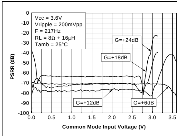
Figure 16. PSRR vs. common mode input voltage
