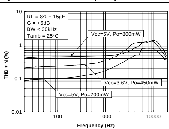
Figure 27. THD+N vs. frequency
