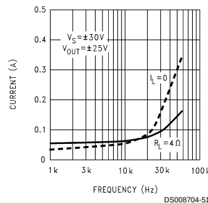
Cross-Supply Current
