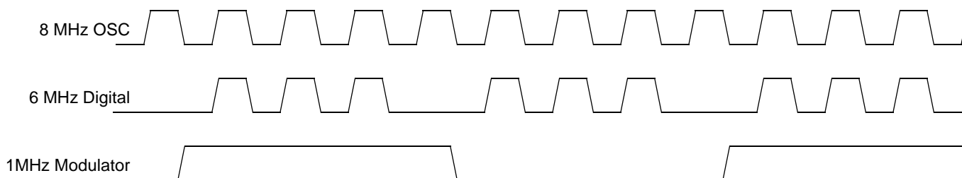
Figure 13. Clock Generation
