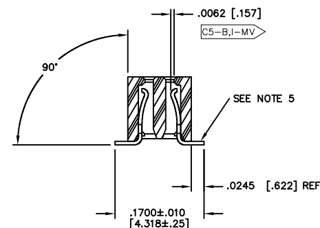
SECT "B-B"
