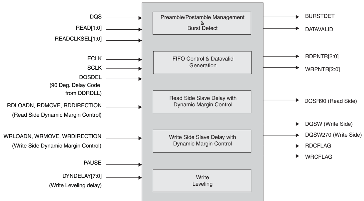
Figure 2-23. DQS Control & Delay Block (DQSBUF)
