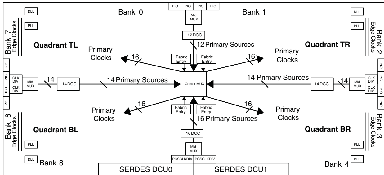
Figure 2-5. LFE5UM-85 Clocking
