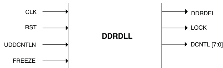
Figure 2-9. DDRDLL Functional Diagram
