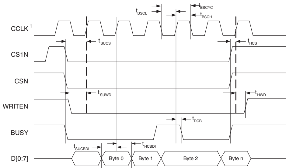
Figure 3-14. sysCONFIG Parallel Port Write Cycle
