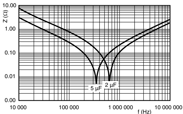
Impedance as function of frequency for box length 44.0 mm (typical curve)
