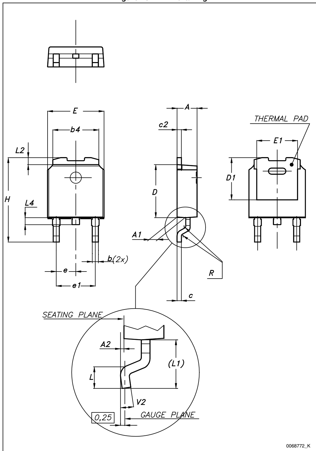
Figure 23. DPAK drawing
