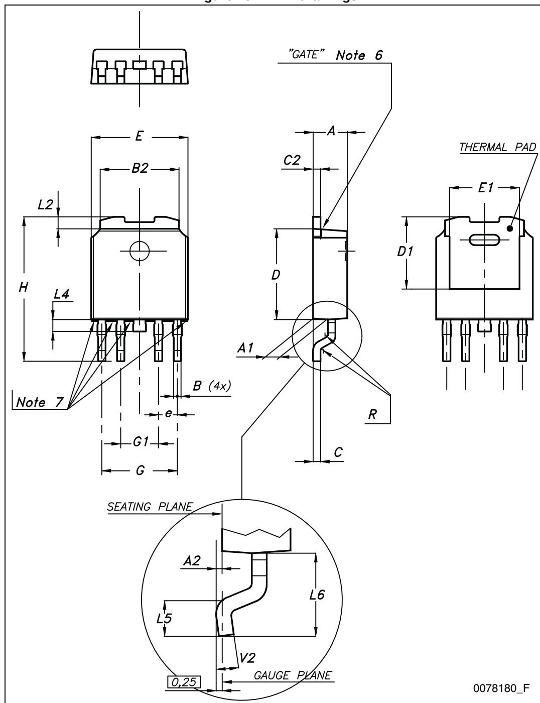
Figure 25. PPAK drawings
