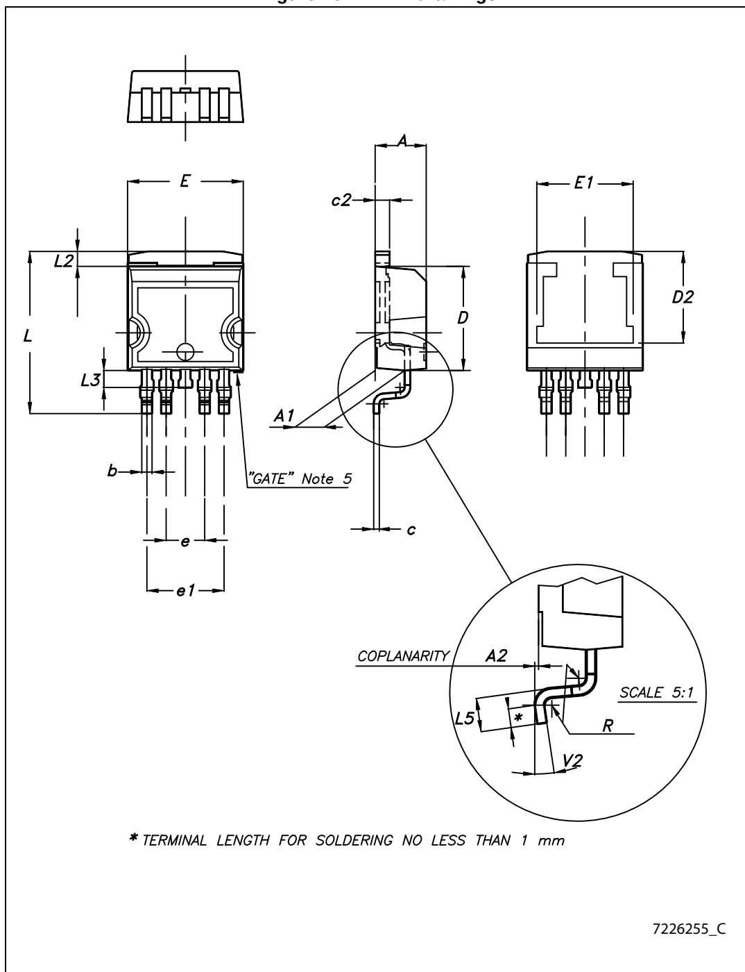
Figure 26. P 2 PAK drawings
