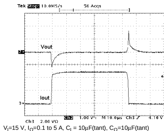
Figure 26: Load Transient
