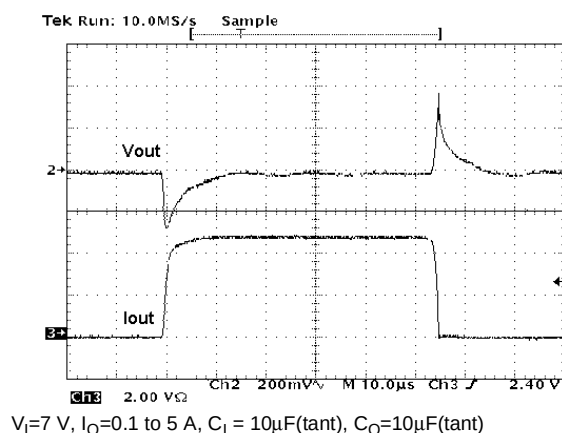
Figure 26: Load Transient
