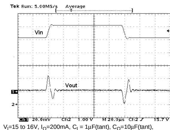
Figure 24: Line Transient
