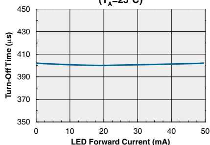
LCA717 Typical Turn-Off vs. LED Forward Current ( T_A=25^\circ\text{C} )
