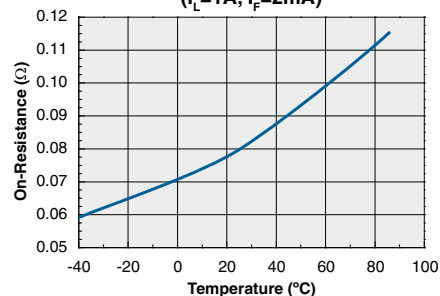
LCA717 Typical On-Resistance vs. Temperature ( I_L=1\text{A} , I_F=2\text{mA} )
