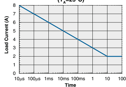
LCA717 Energy Rating Curve ( T_A=25^\circ\text{C} )
