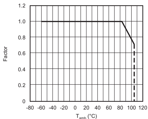
RMS voltage in function of temperature
