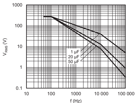
Maximum RMS voltage as function of frequency T_{amb} \leq 85^\circ\text{C} ; U_n = 275\text{ V}_{AC}
