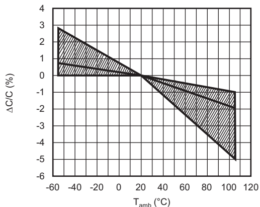
Capacitance as a function of ambient temperature (typical curve)
