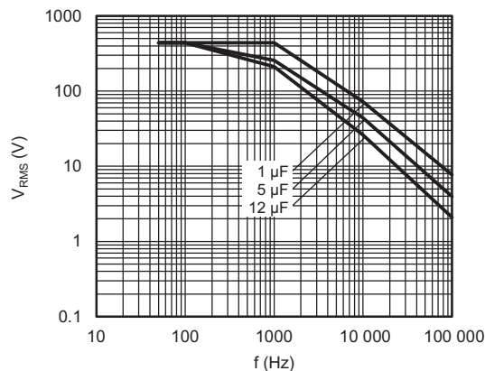
Maximum RMS voltage as function of frequency T_{amb} \leq 85^\circ\text{C} ; U_n = 440\text{ V}_{AC}
