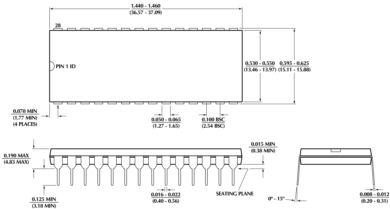
Package: P28W 28-Pin Wide PDIP
