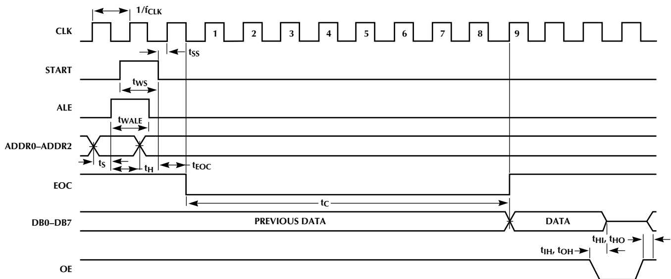
Figure 5. Timing Diagram
