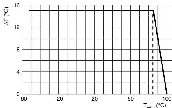
Maximum allowed component temperature rise ( \Delta T ) as a function of the ambient temperature ( T_{\text{amb}} )
