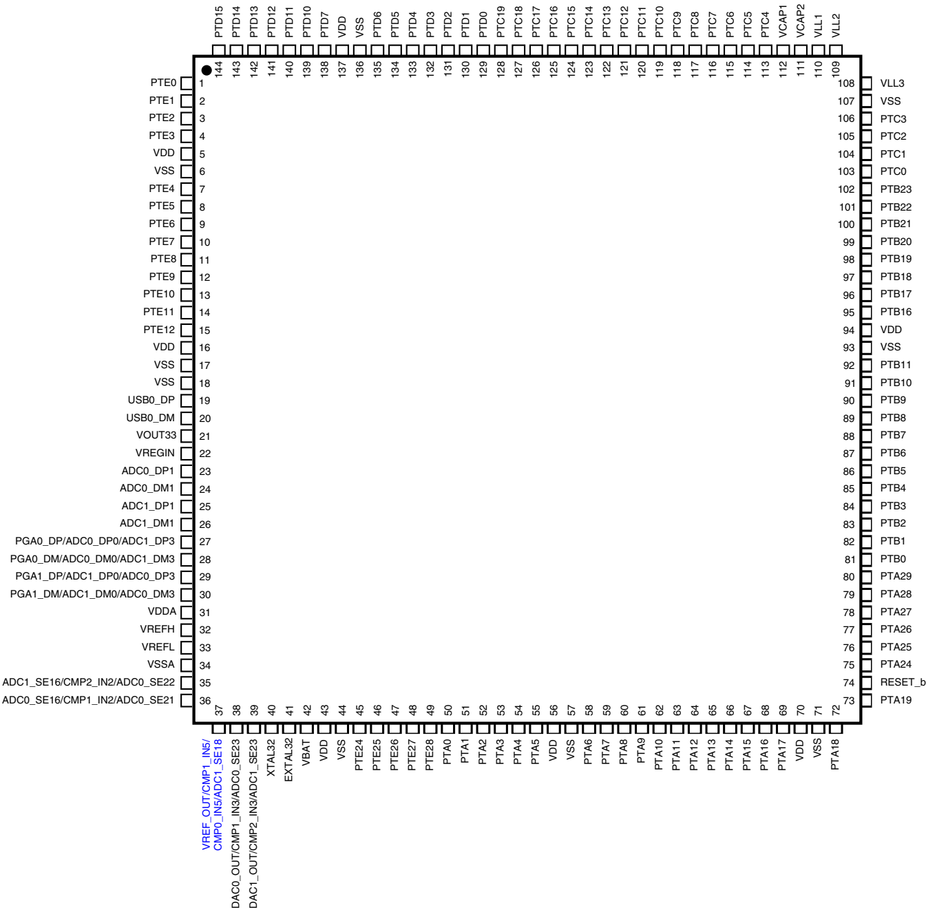
Figure 28. K40 144 LQFP Pinout Diagram
