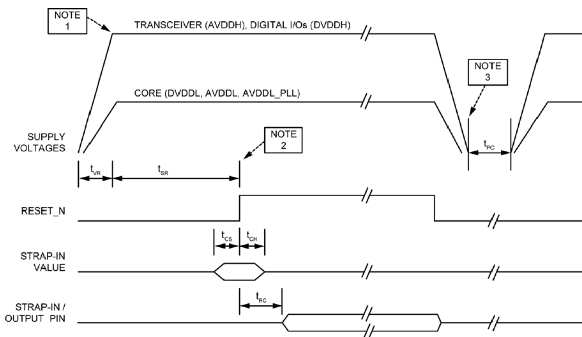
Figure 19. Power-Up/Power-Down/Reset Timing
