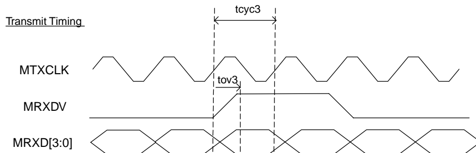
Figure 16. MAC Mode MII Timing—Data Transmitted from MII
