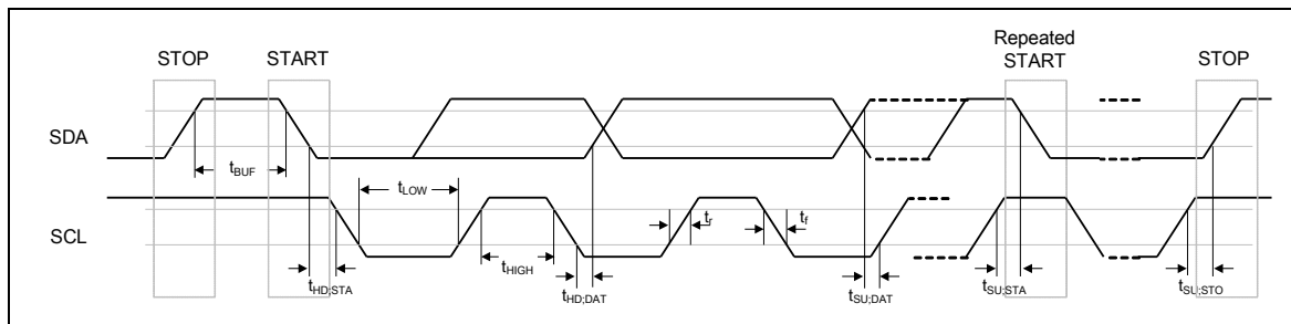
Figure 5.9-1 Bus Timing
