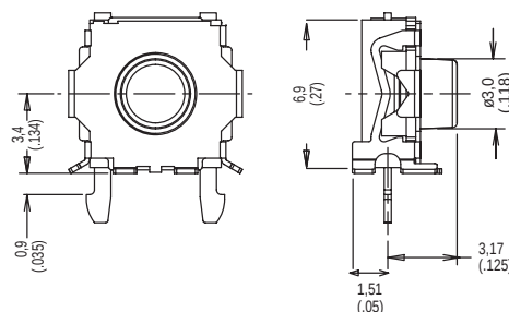
PAD LAYOUT
