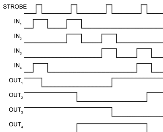
Unipolar 2-Phase Drive
