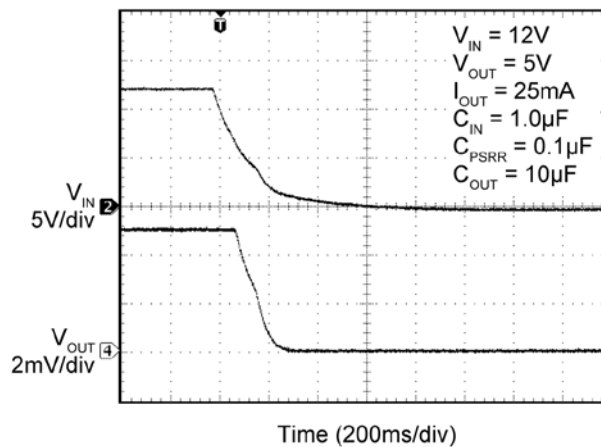
Soft Turn-Off
