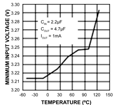
Minimum Input Voltage vs. Temperature
