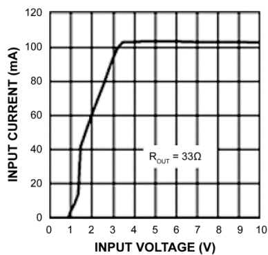
Input Current vs. Input Voltage (3.3V Version)
