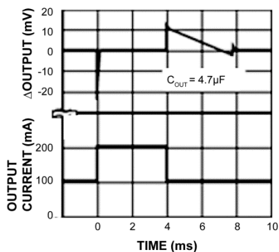
Load Transient
