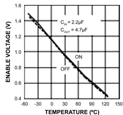
Enable Voltage Threshold vs. Temperature
