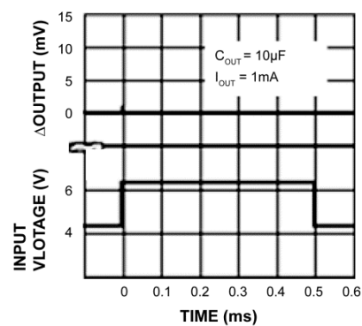
Line Transient
