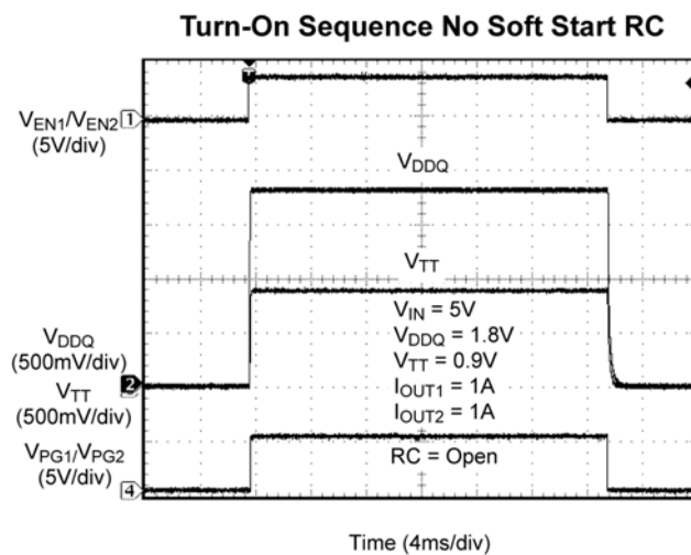
Figure 7. V_{TT} Turn-On without Delay
