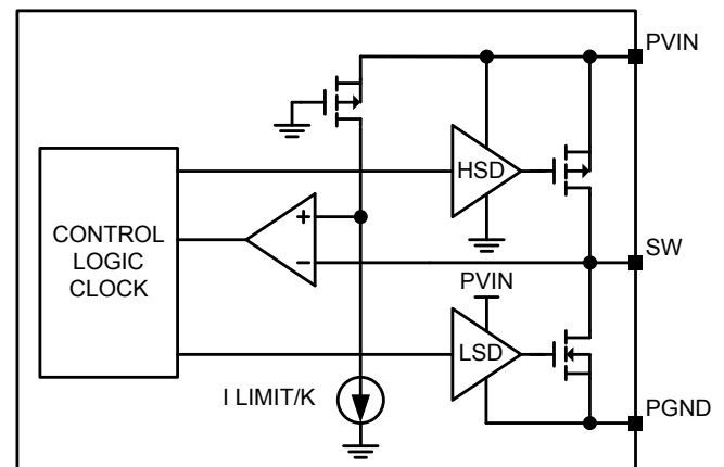
Figure 5. Current-Limit Detail
