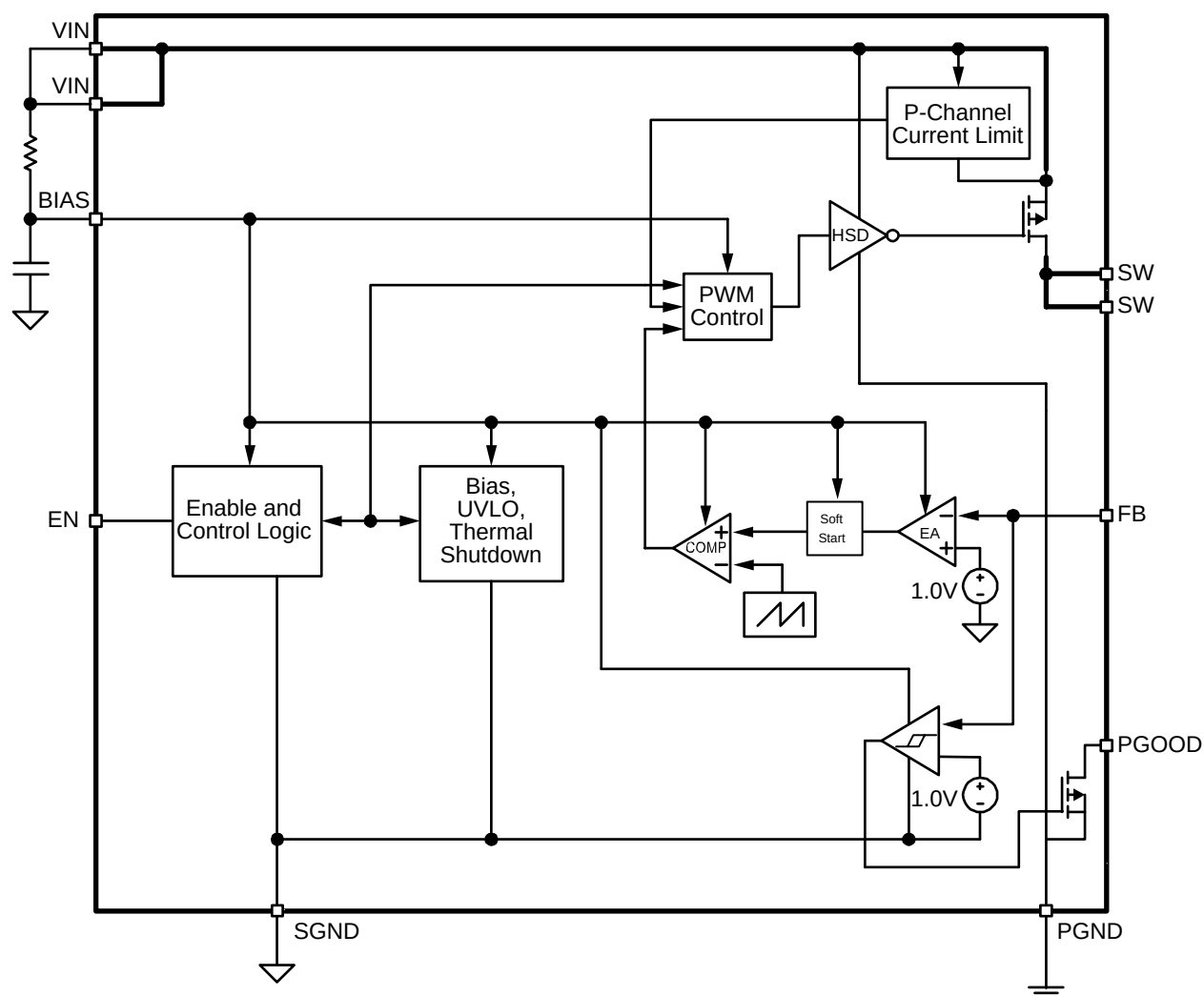
MIC4723 Block Diagram
