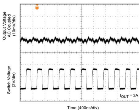
Output Ripple
