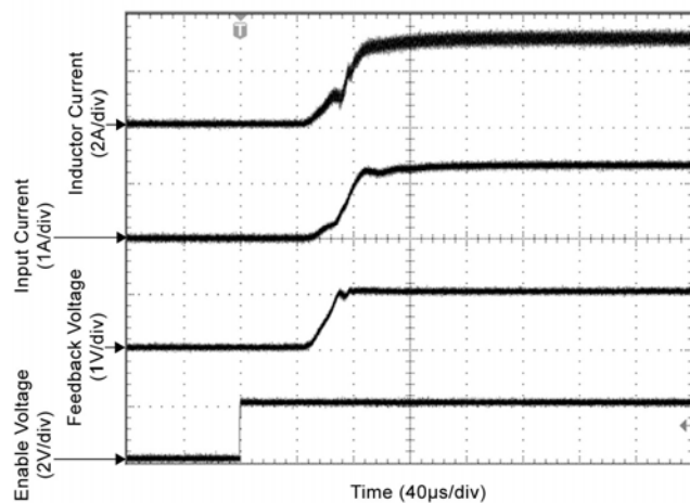
Start-Up Waveforms
