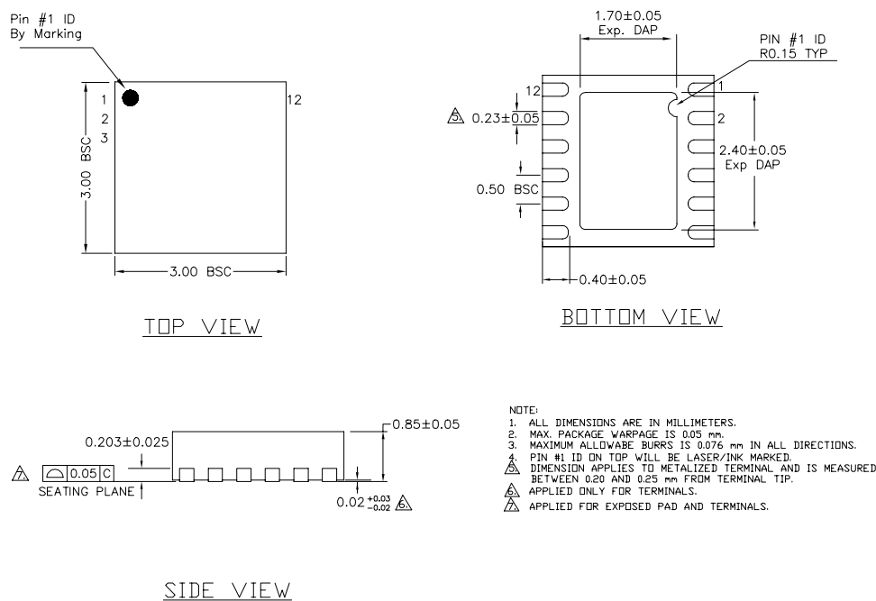
12-Pin 3mm x 3mm MLF® (ML)
