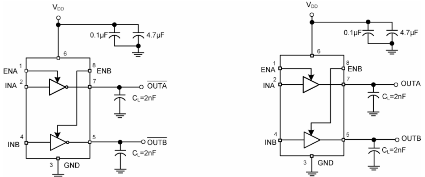
Figure 1. Test Circuit
