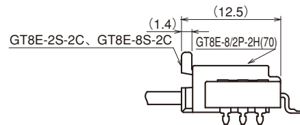
◆Fitting diagram
