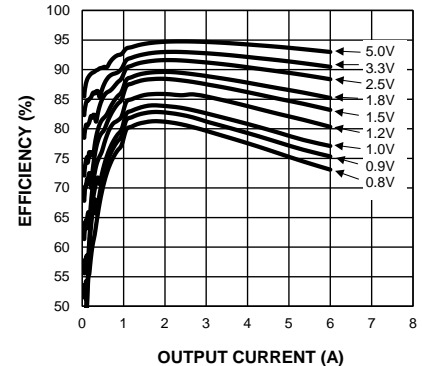
Efficiency ( V_{IN} = 12V ) vs. Output Current
