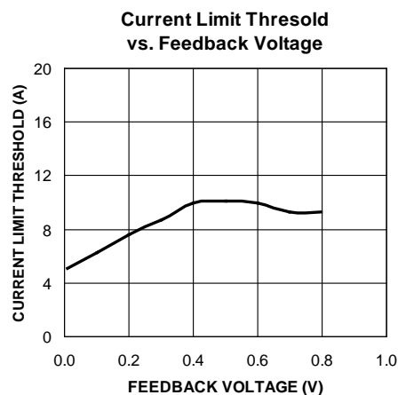
Figure 5. MIC24052 Current-Limit Foldback Characteristic
