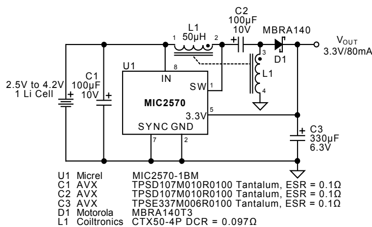
Example 4. Single Cell Lithium to 3.3V/80mA Regulator
