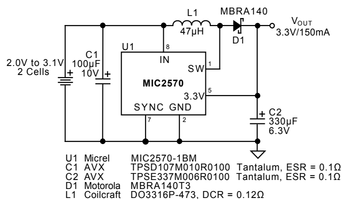
Example 2. 3.3V/150mA Regulator
