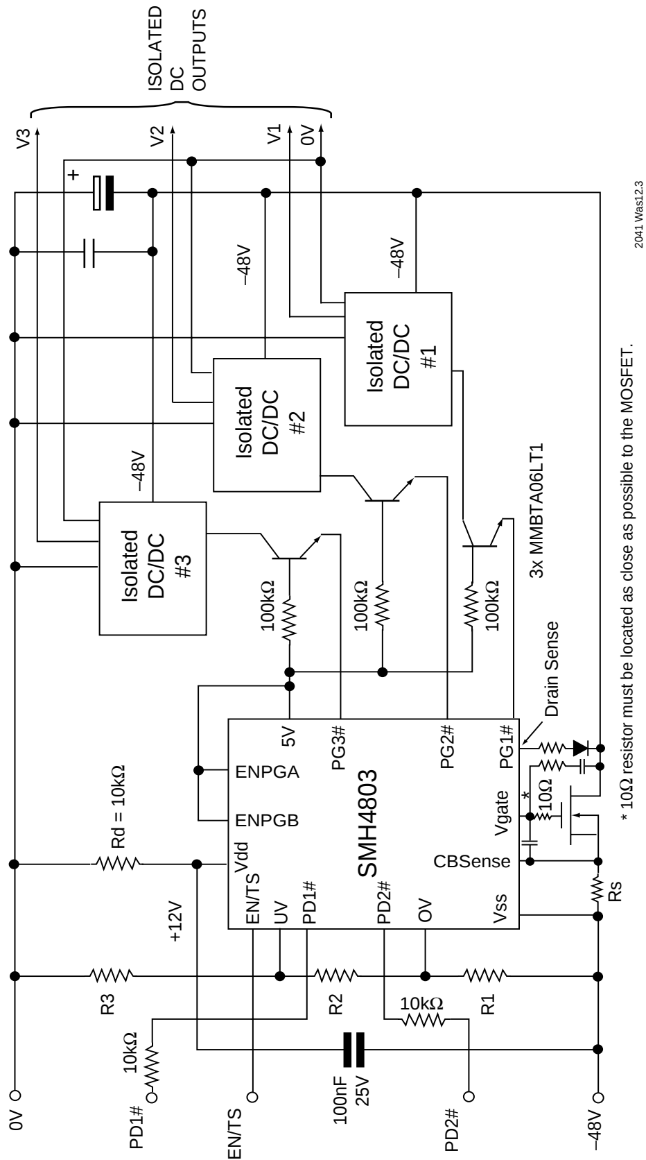
Figure 9. Typical Application Sequencing 3 DC/DC Converters
