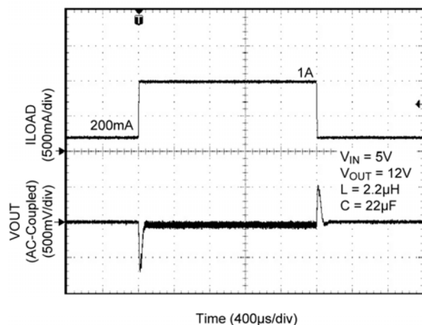
Load Transient (12V Output)
