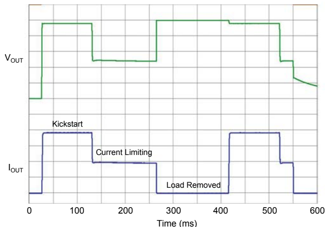
Figure 9. Kickstart
