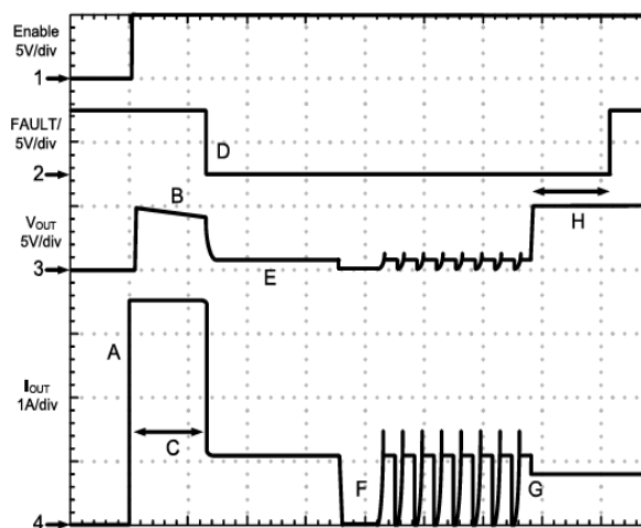
Figure 3. Kickstart Operation
