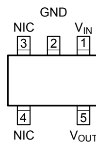
SOT 23-5 (M5) Top View
