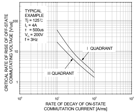
Figure 16. Commutation Characteristics
