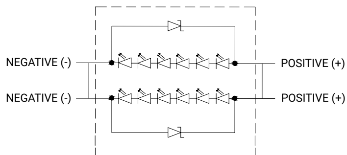
18-V Configuration
