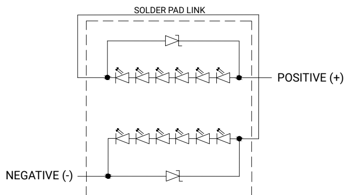
36-V Configuration
