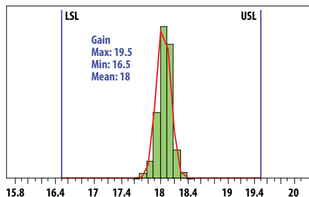
Figure 4. Gain @ 2.5GHz, 5V, 56mA Mean = 18
