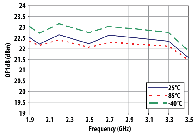
Figure 24. OP1dB vs Frequency vs Temperature
