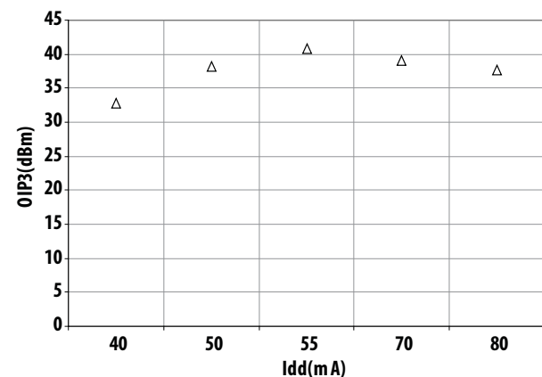
Figure 12. OIP3 vs Idd at 5V Tuned for Optimum OIP3 and Fmin at 2GHz.
