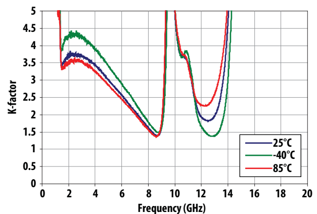
Figure 26. K-factor vs Frequency vs Temperature
