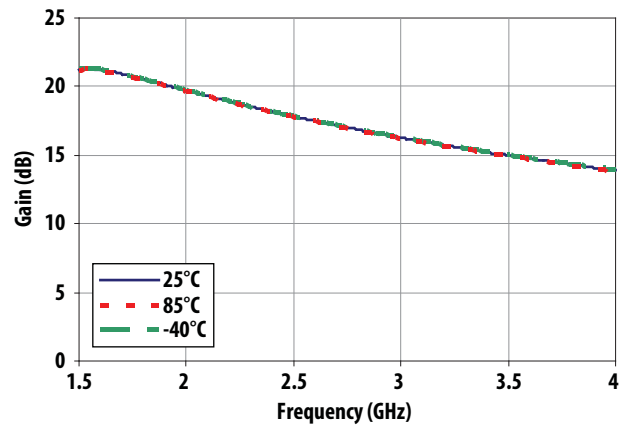
Figure 22. Gain vs Frequency vs Temperature
