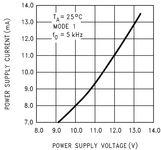
Power Supply Current vs. Power Supply Voltage
