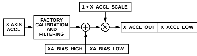
Figure 23. User Calibration Signal Path, Gyroscopes
