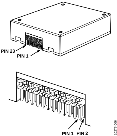
Figure 6. Axial Orientation (Top Side Facing Up)
