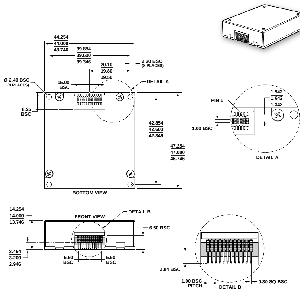
Figure 31. 24-Lead Module with Connector Interface [MODULE] (ML-24-6)
