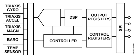
Figure 12. Basic Operation
